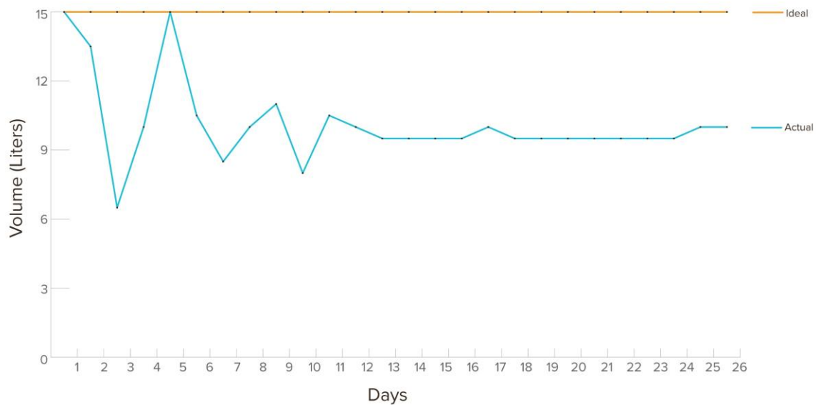
Figure 1. The amount of fresh water generated by the solar desalination tool
